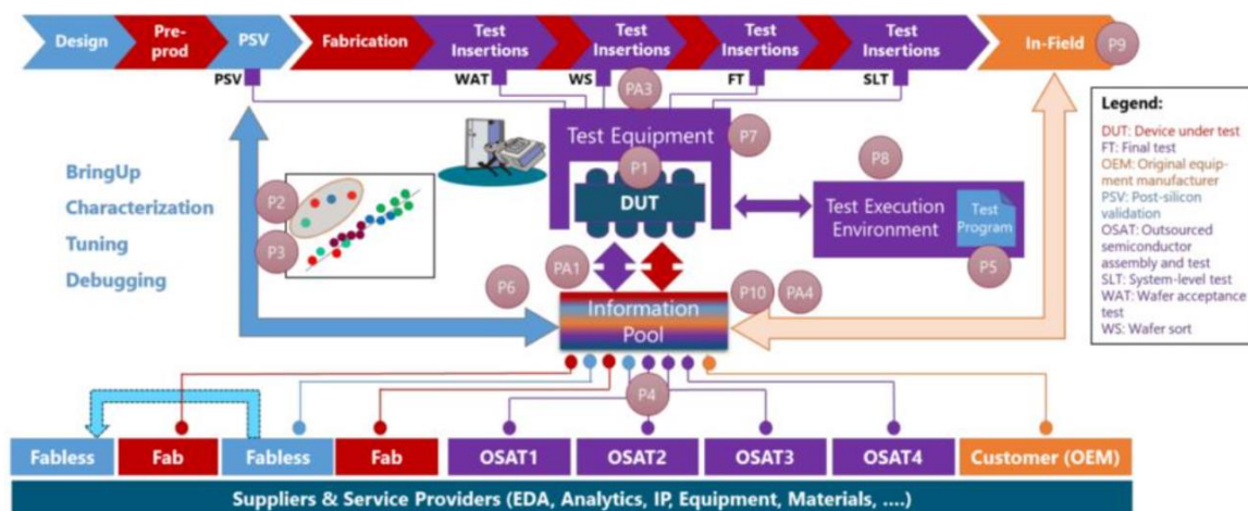
圖 5. Semiconductor wafer manufacturing to packaging and testing
